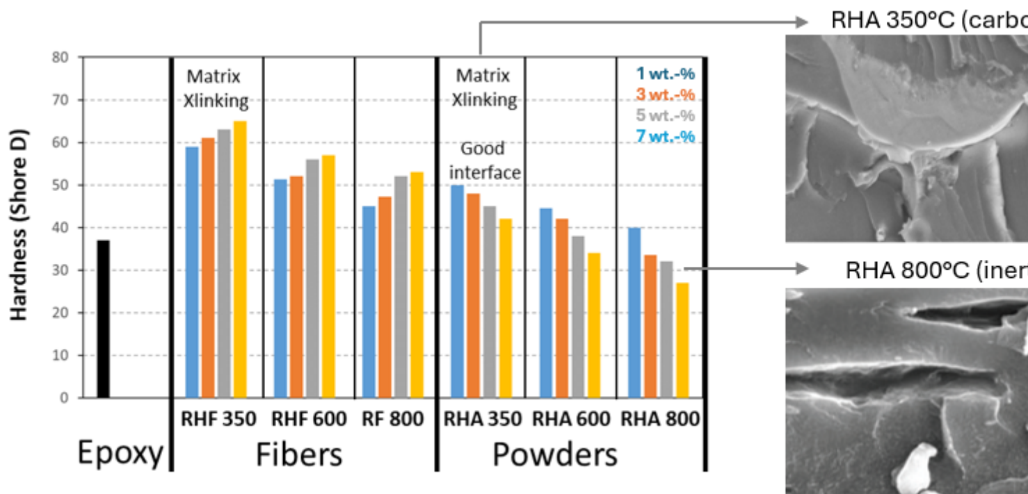
Figure 3. Experimental testing results of coating properties (e.g. hardness as a general measure for mechanical resistance) containing epoxy binder and pyrolyzed rice-husk fibres (RHF) or rice husk powders (RHA) at different temperatures and added at 1 to 7 wt.-% concentration.
