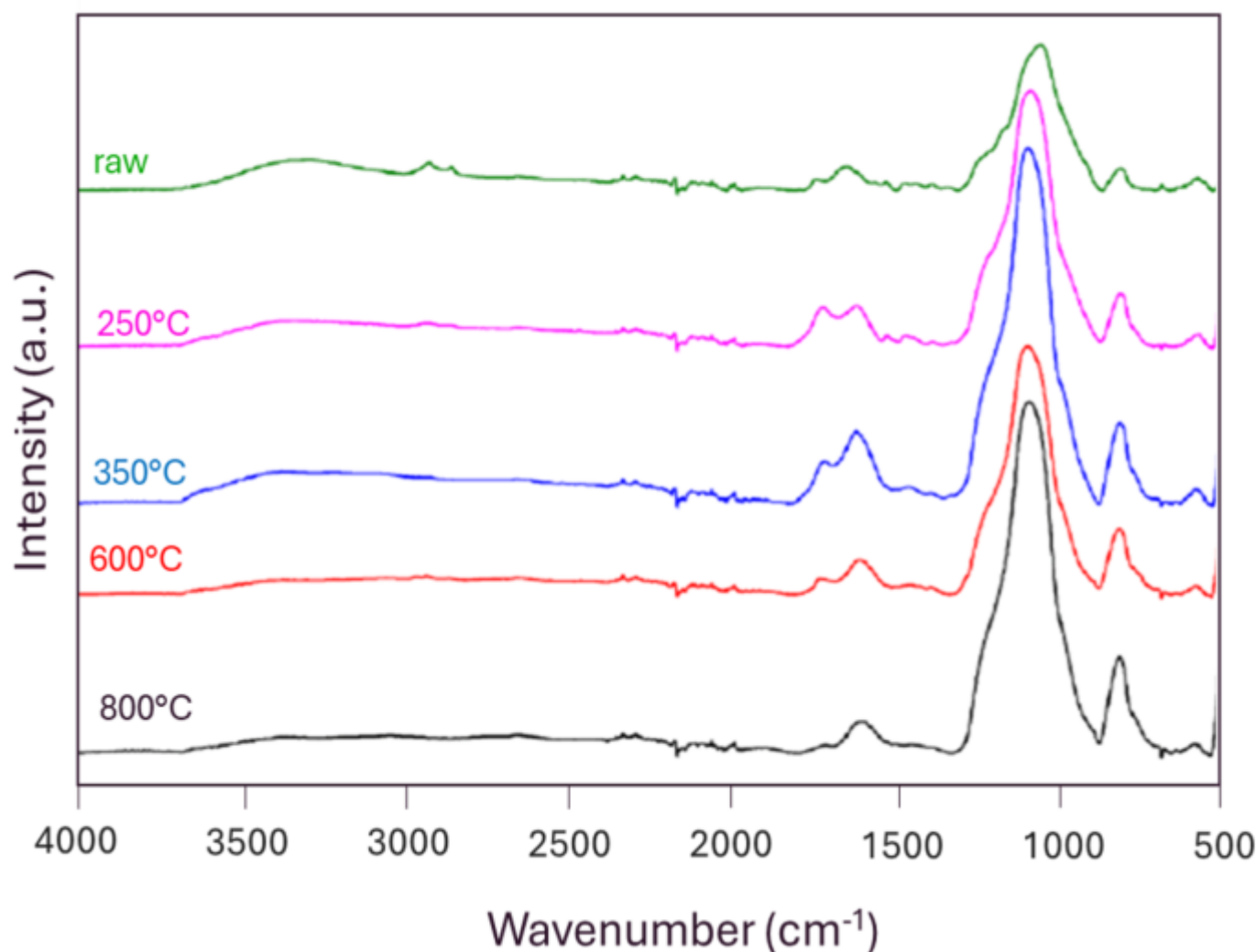
Figure 1. Characteristics of pyrolysed rice husk at laboratory scale under different temperatures, including FTIR analysis, macroscopic pictures and microscopic morphology.
