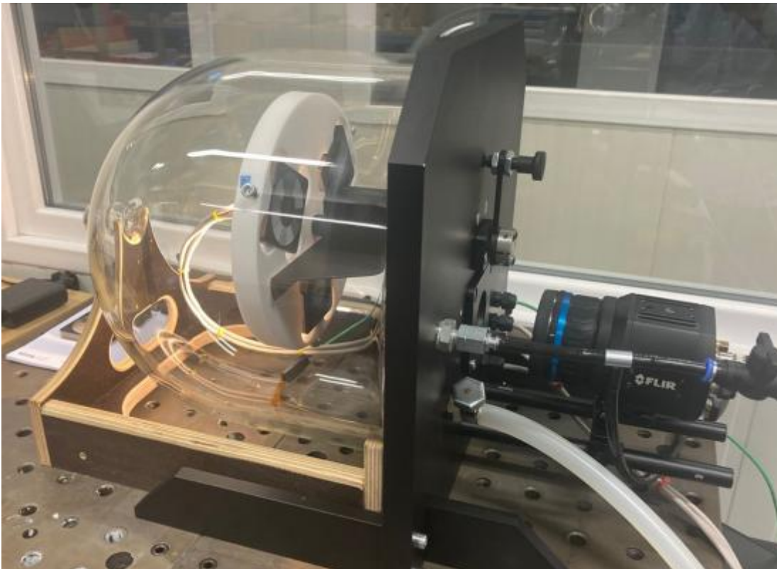
Figure 1: Vacuum clock with IR camera and samples
