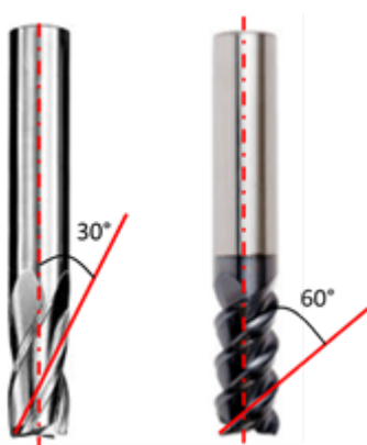
End mills with 30° and 60° helix angles
